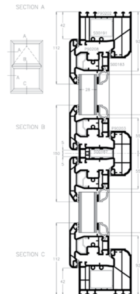
Storm 2 72mm outer frame (large)
