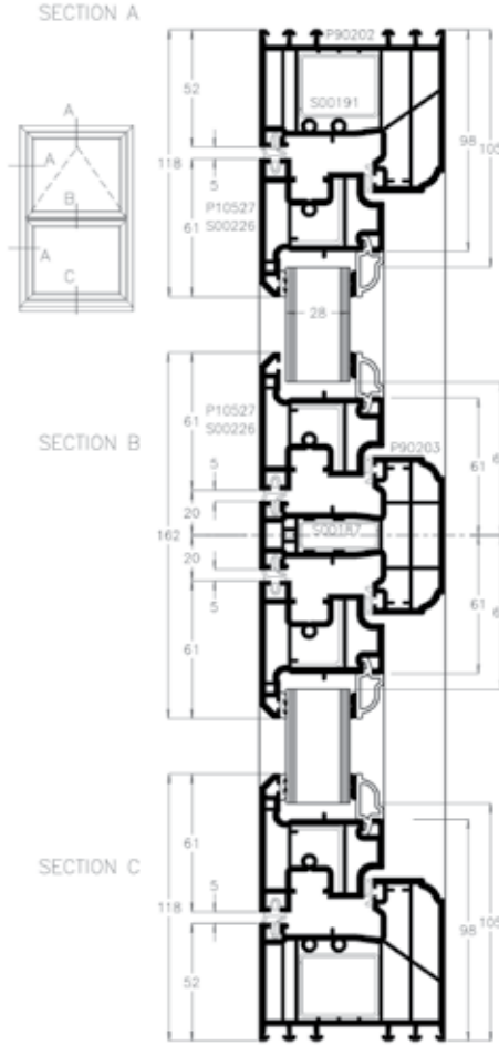
Flush 72mm outer frame (large)
