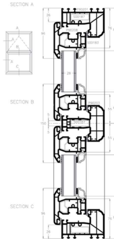
Storm 2 56mm outer frame (small)
